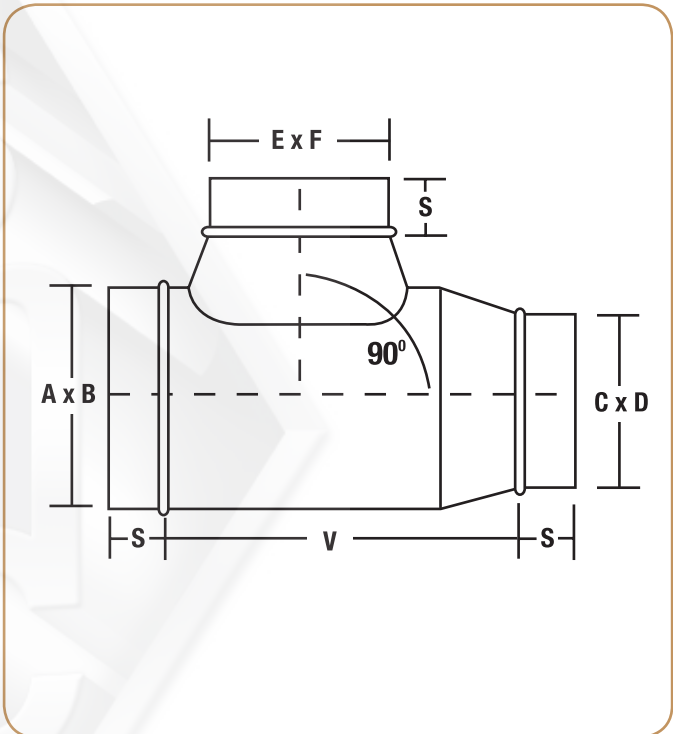
Reducing Conical Tee
