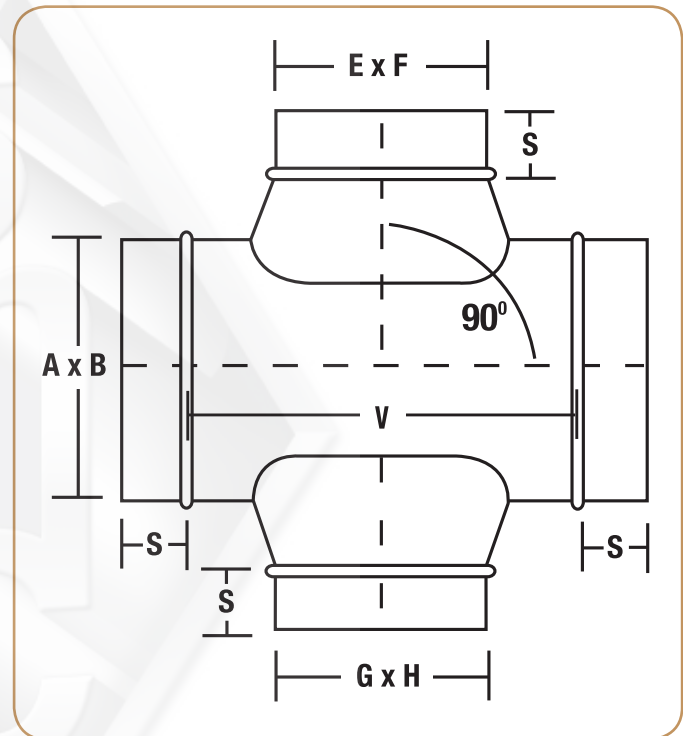
Conical Cross
