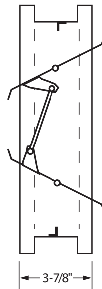
Model: OBS Opposed Blade Sealed Damper
